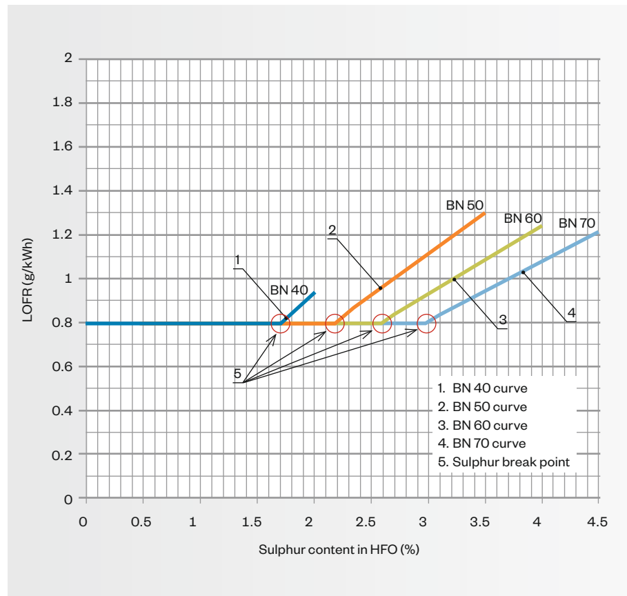
■ Fig. 2 – Recommended feedrate adjustments at loads <60%, based on fuel sulphur content (S%) and cylinder oil in use.
