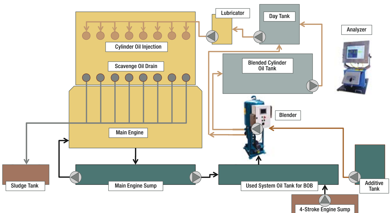
■ Fig. 6 - The principle of the Blending on Board system.
