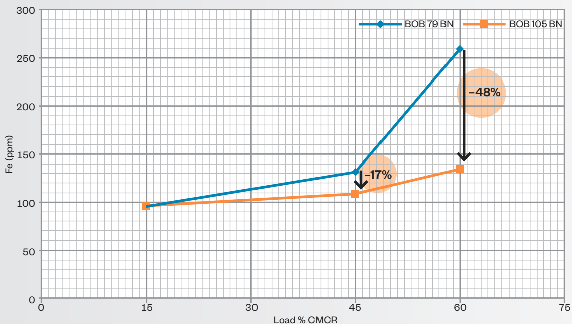
Total Iron content of piston underside drain oil during operation with BOB cylinder lubricant.
