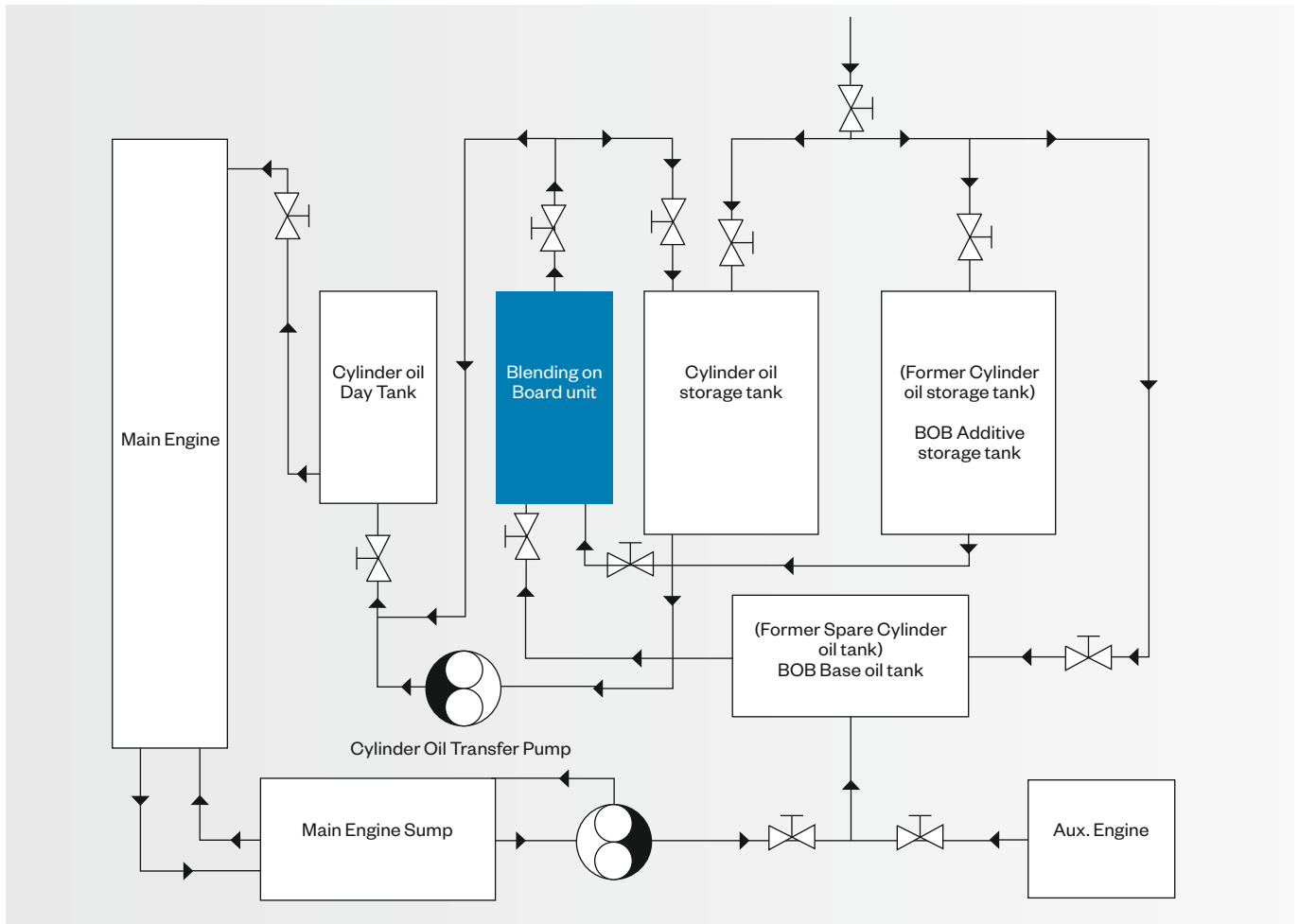
■ Fig. 7 – The layout and flow diagram of the Blending on Board system.
