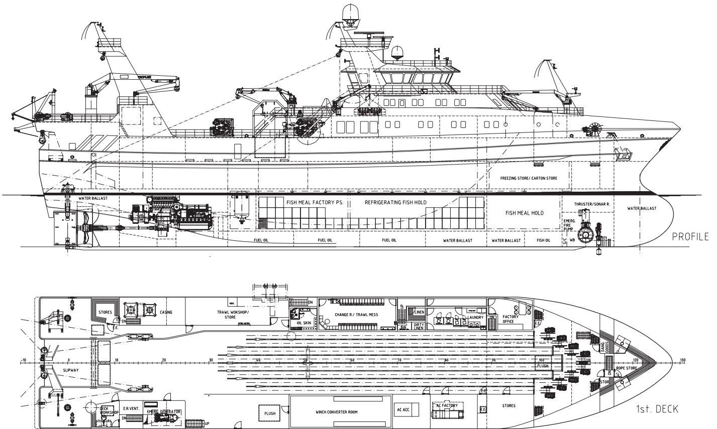
Fig.1 Detailed elavation drawings
