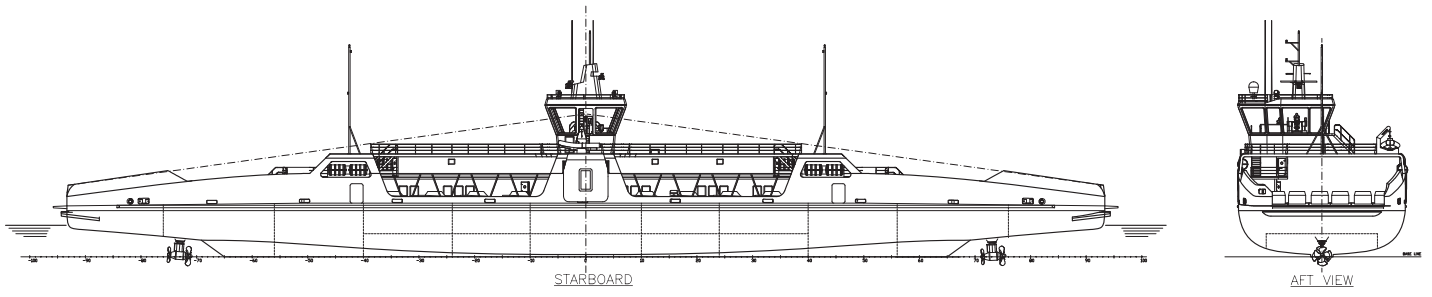
Fig.1 Detailed elevation drawings
